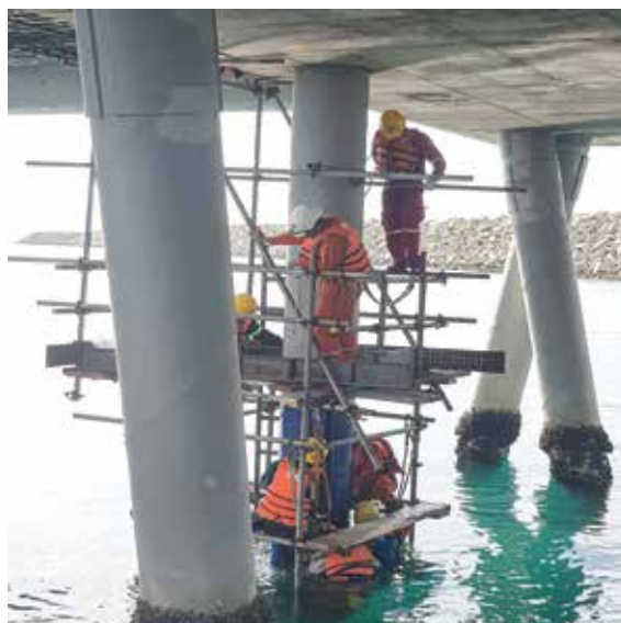
PROTECTING THE JETTY PILES OF DUNG QUAT REFINERY
